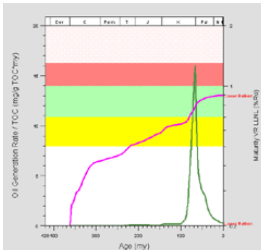
BAKKEN SOURCE ROCK OIL PLAY, MCKENZIE COUNTY, NORTH DAKOTA, COURTESY R. COSKEY
